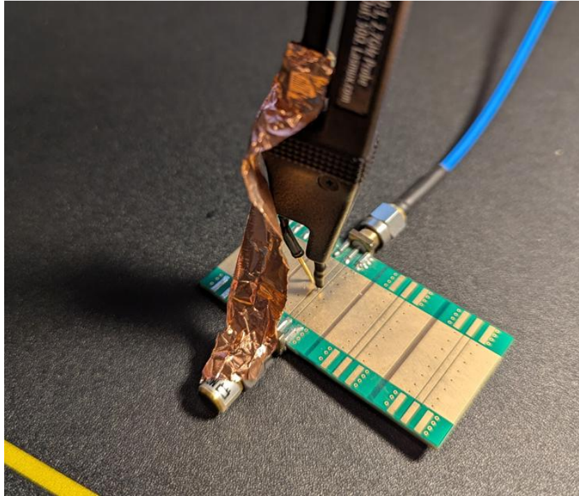
Figure 7. Using copper tape to enhance the grounding of the probe, for when probe is not used handheld.
