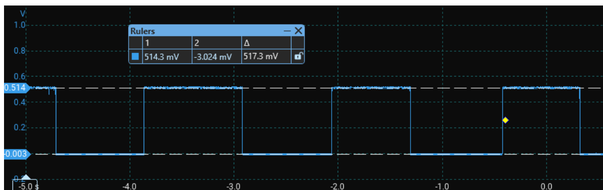
Figure 5. Low frequency and higher voltage performance. Probe response of an 0.5 Hz, 10 V square wave.
