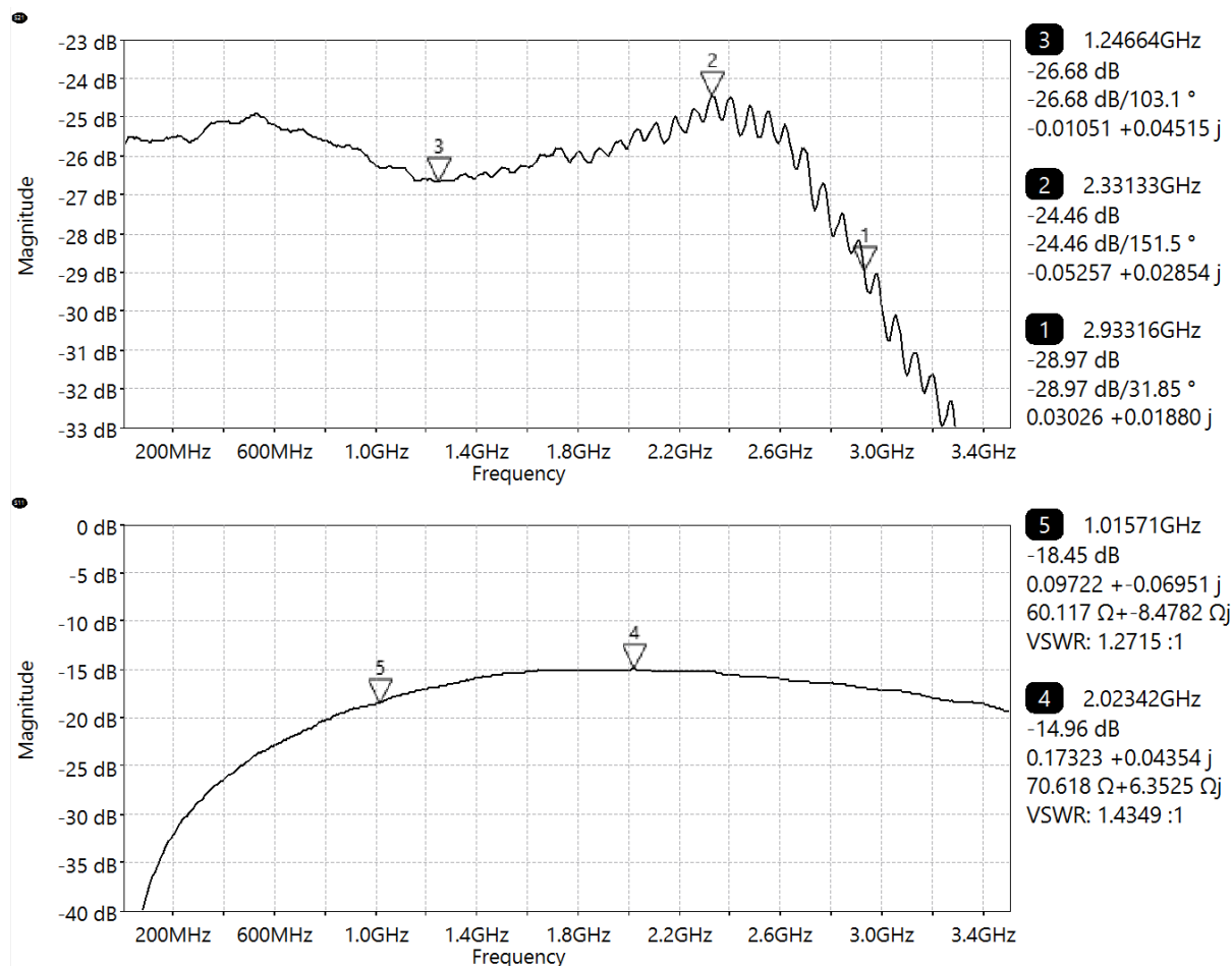
Figure 1. Top: Probe frequency response. Typical attenuation is -26 dB. Bottom: 50 Ω coplanar waveguide with probe attached return loss.
