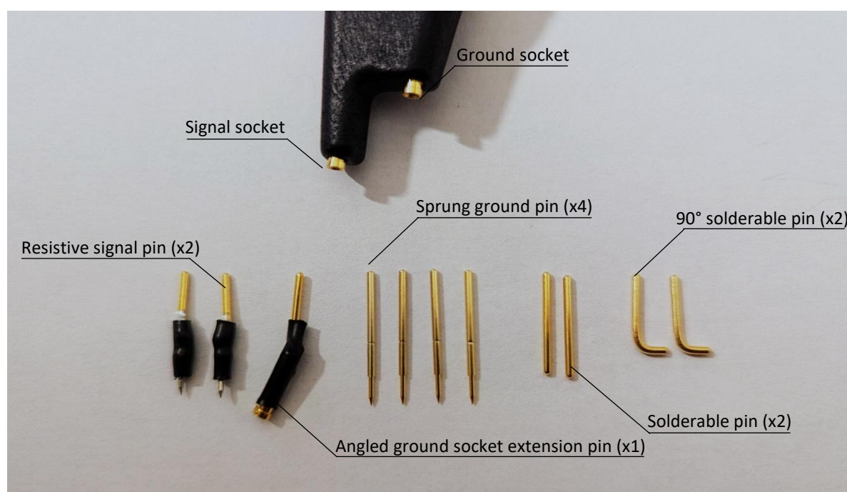
Figure 8. Supplied pins with probe.
